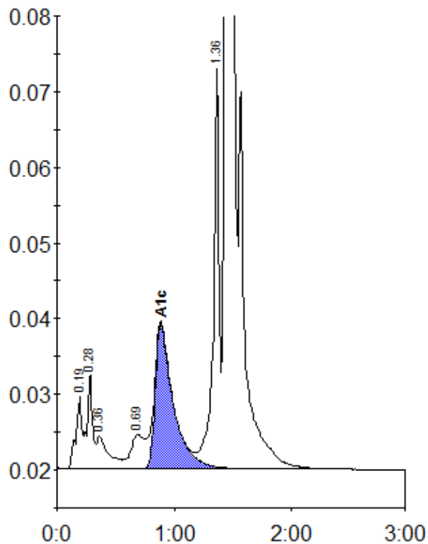
Peak table - ID: 10633791
